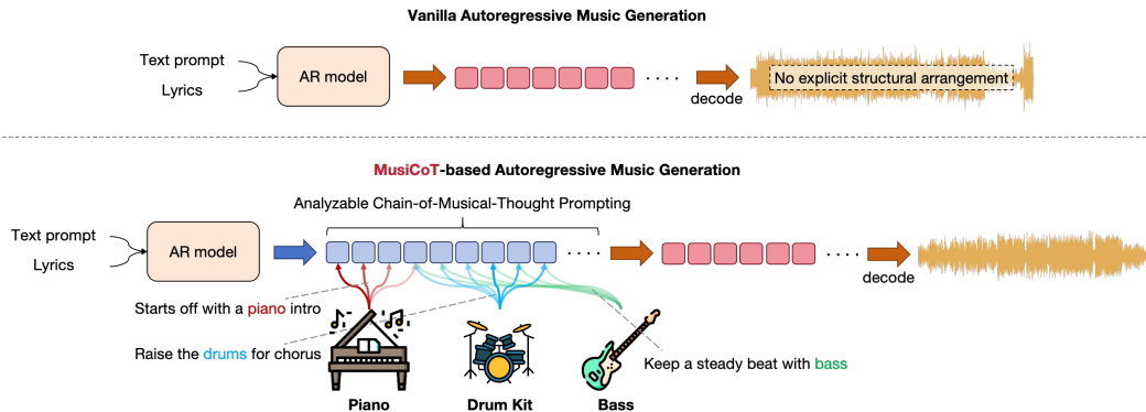
Figure 1: This illustration showcases the MusiCoT reasoning process for music generation, focusing on instrumental arrangement. The arrows are color-coded to indicate the intensity of each instrument: darker colors represent higher intensity, while lighter shades signify lower intensity.
